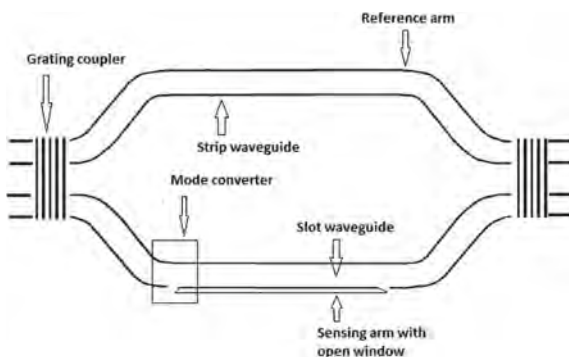
Fig. 2 Schematic view of Mach–Zehnder interferometer based on slot waveguide. Reproduced from Ref. [13]
