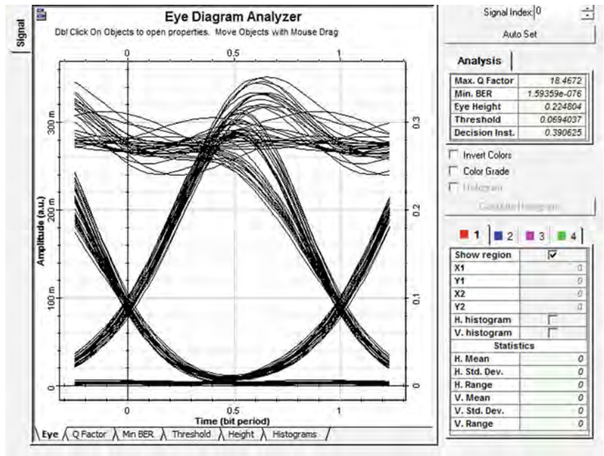
Fig. 3 Simulated result of eye-diagram after CFBG dispersion compensation
