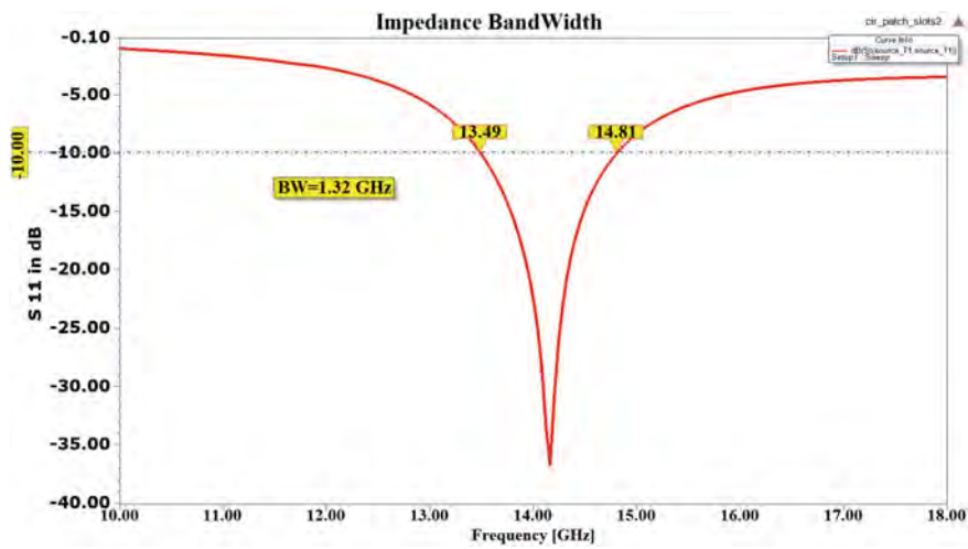
Fig. 2 S parameter versus frequency plot of propounded patch in dB
