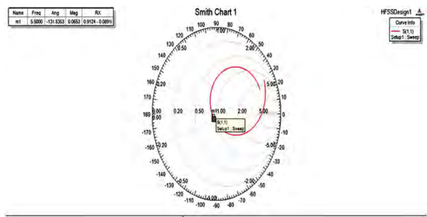
Fig. 12 Simulation result of Smith chart without DGS
