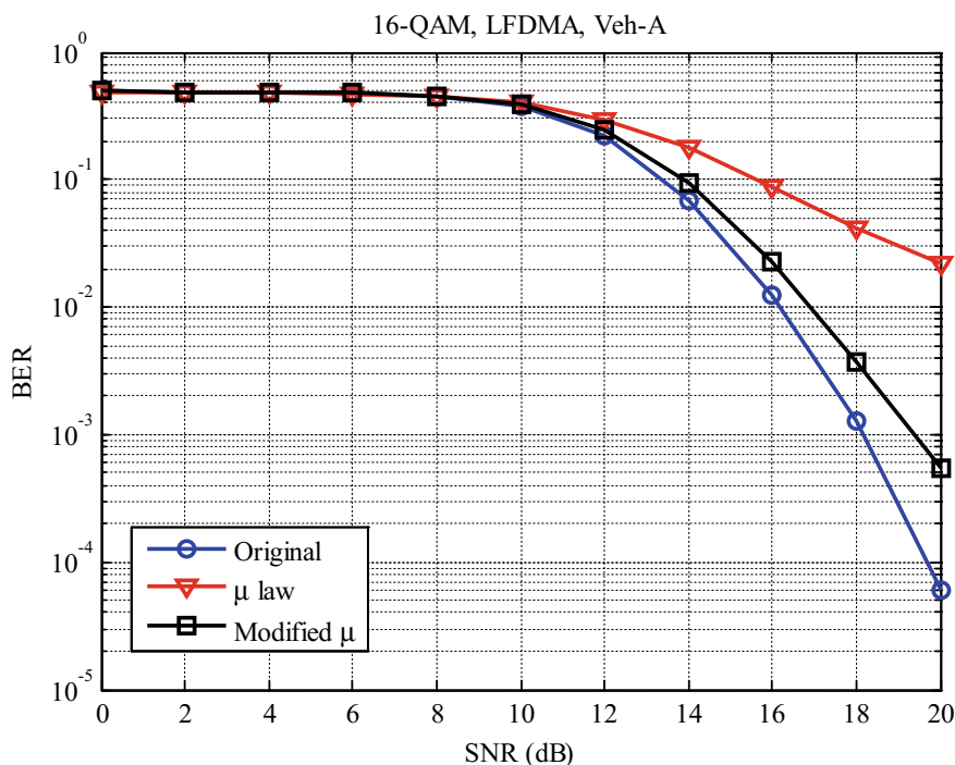
Fig. 6 BER curves of companded and original systems over Vehicular-A channel
