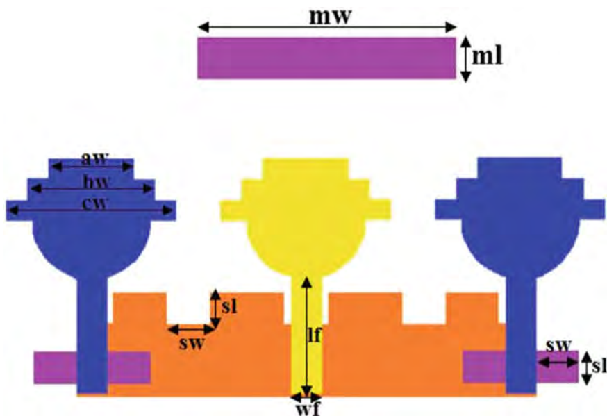
Fig. 3 Antenna array with parasitic element
