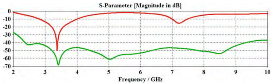
Fig. 4 S-parameters comparison
