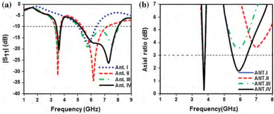
Fig. 3 Comparisons of different configurations Ant. I–IV, a |S_{11}| , and b AR
