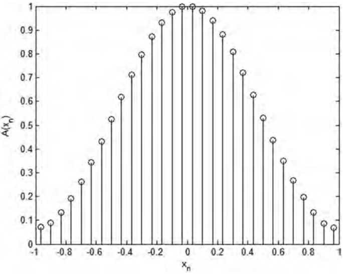
Fig. 14 Amplitude excitation coefficients obtained by PSO method for N = 30 element array
