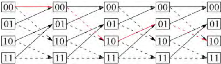
Fig. 7 Trellis diagram
