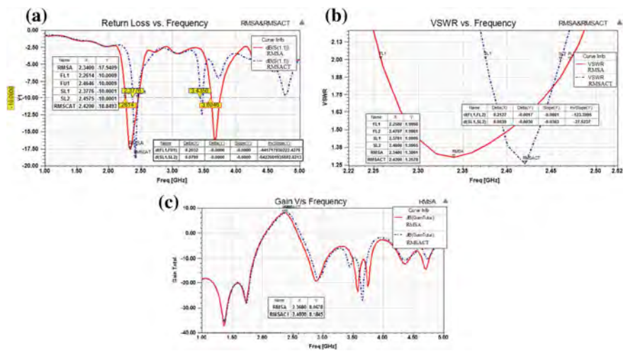
Fig. 4 a Simulated return loss. b Simulated VSWR. c Gain versus frequency
