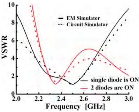
Fig. 2 VSWR of antenna when a single diode is turned ON, b any two diodes are turned ON where solid and dotted lines present EM simulation and circuit simulation results, respectively
