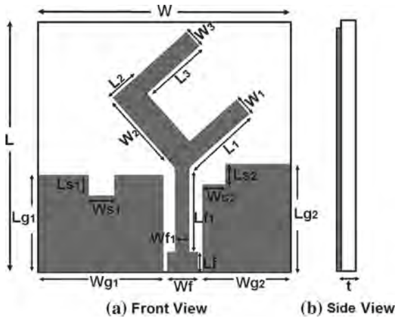
Fig. 1 Configuration of the proposed offset CPW-fed tilted asymmetrical U-shaped patch-printed antenna. The detailed dimensions of the antenna are L = 33 , W = 34 , W_l = 2.5 , L_1 = 11.5 , W_2 = 11.9 , L_2 = 4.2 , W_3 = 2.4 , L_3 = 9.4 , L_{g1} = 11 , L_{g2} = 12 , W_{g1} = 17.65 , W_{g2} = 12.65 , L_{s1} = 4 , W_{s1} = 5 , L_{s2} = 2 , W_{s2} = 4.65 , L_f = 3 , W_f = 3 , L_{f1} = 9.4 , W_{f1} = 1.5 , t = 1.6 (all dimensions are in mm)
