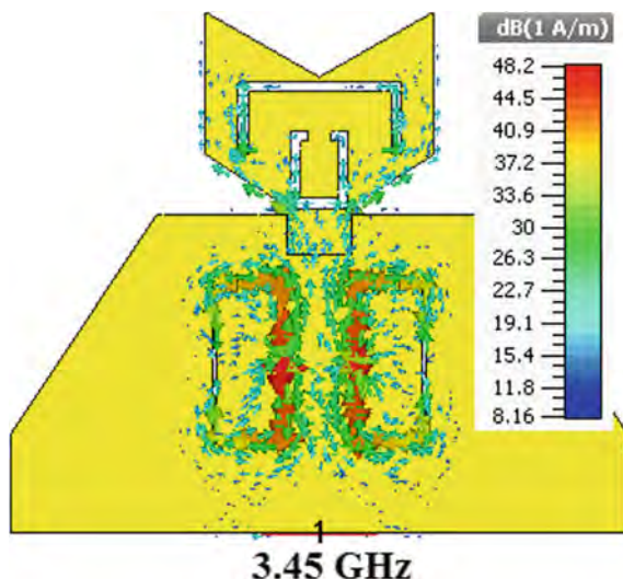
Fig. 5 Surface current distributions for the proposed antenna at 3.45 GHz
