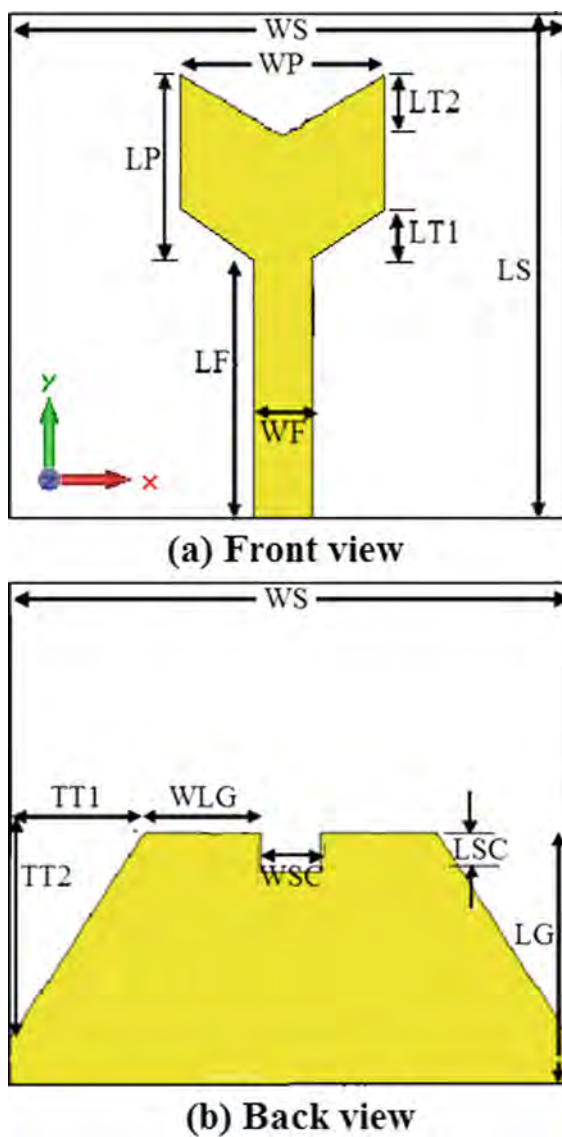
Fig. 1 Basic Y-shaped antenna a front view b back view
