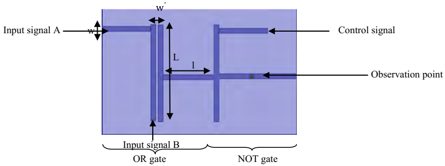
Fig. 4 Schematic of proposed NOR gate with following parameters; w = 50 nm, l = 514 nm, w' = 25 nm, and L = 1000 nm
