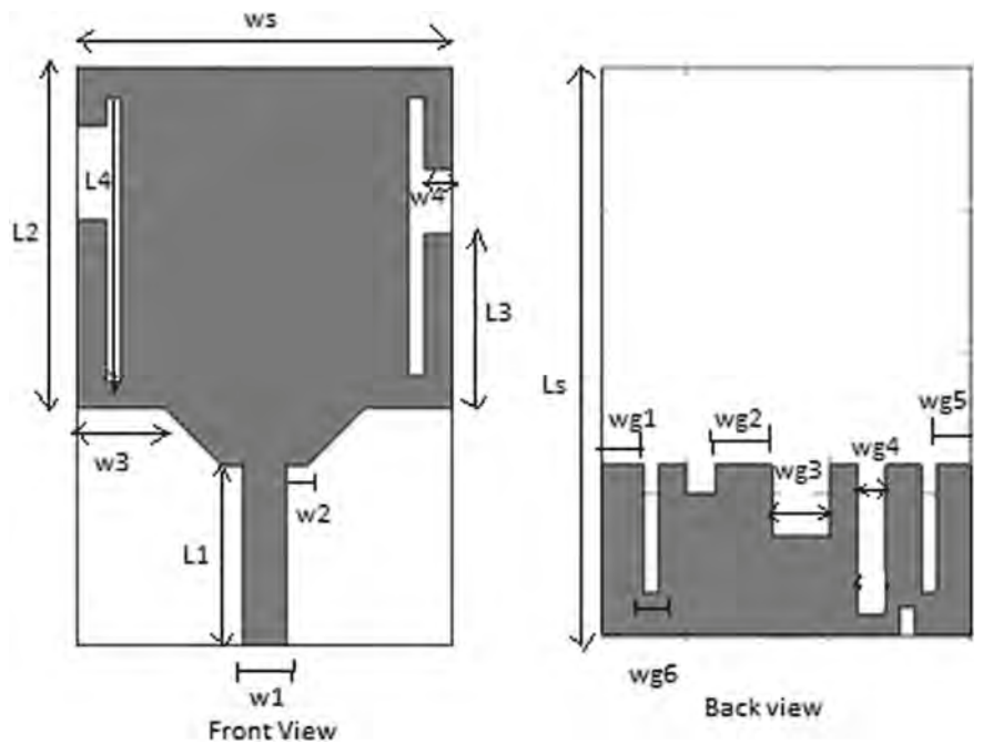
Fig. 1 Front and back view of the proposed antenna
