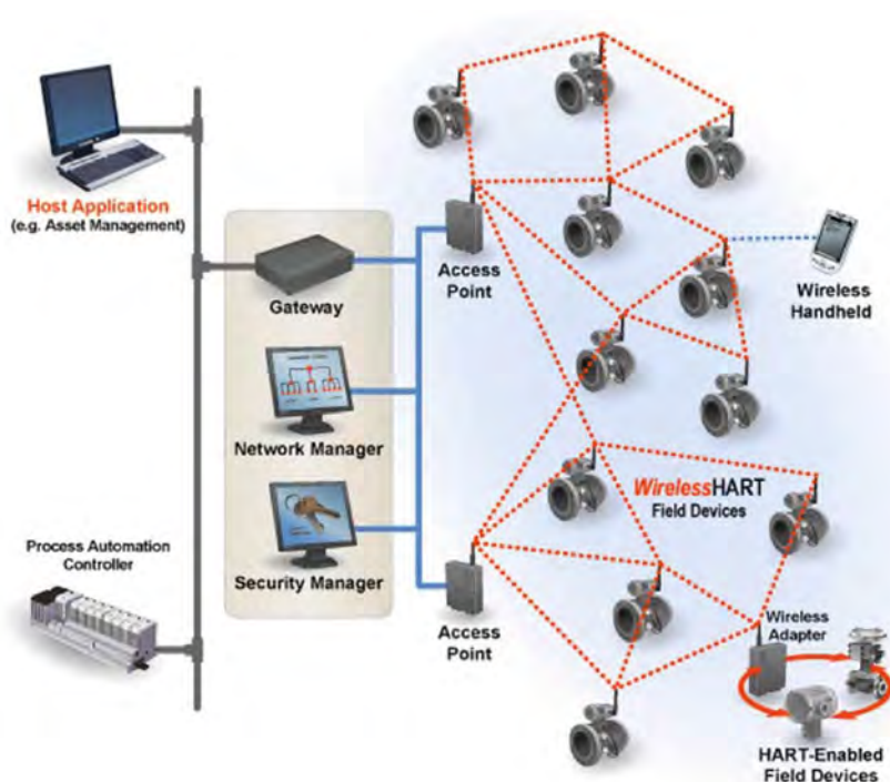
Fig. 6 Architecture of a WirelessHART network. As illustrated in [17, Fig. 1]
