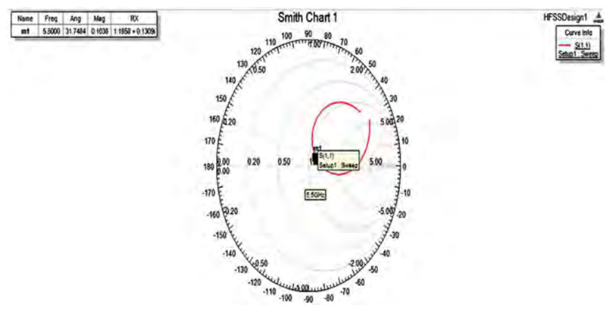
Fig. 13 Simulation result of Smith chart with DGS
