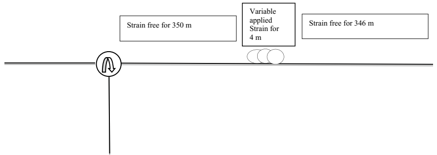
Fig. 2 Structure of SMF under test
