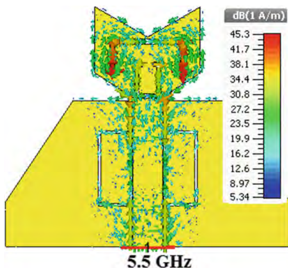
Fig. 6 Surface current distributions for the proposed antenna at 5.5 GHz
