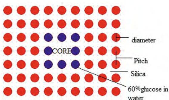
Fig. 1 Cross-sectional view
