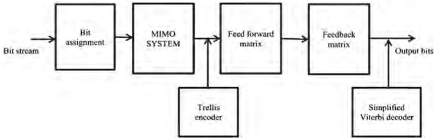
Fig. 8 Block diagram
