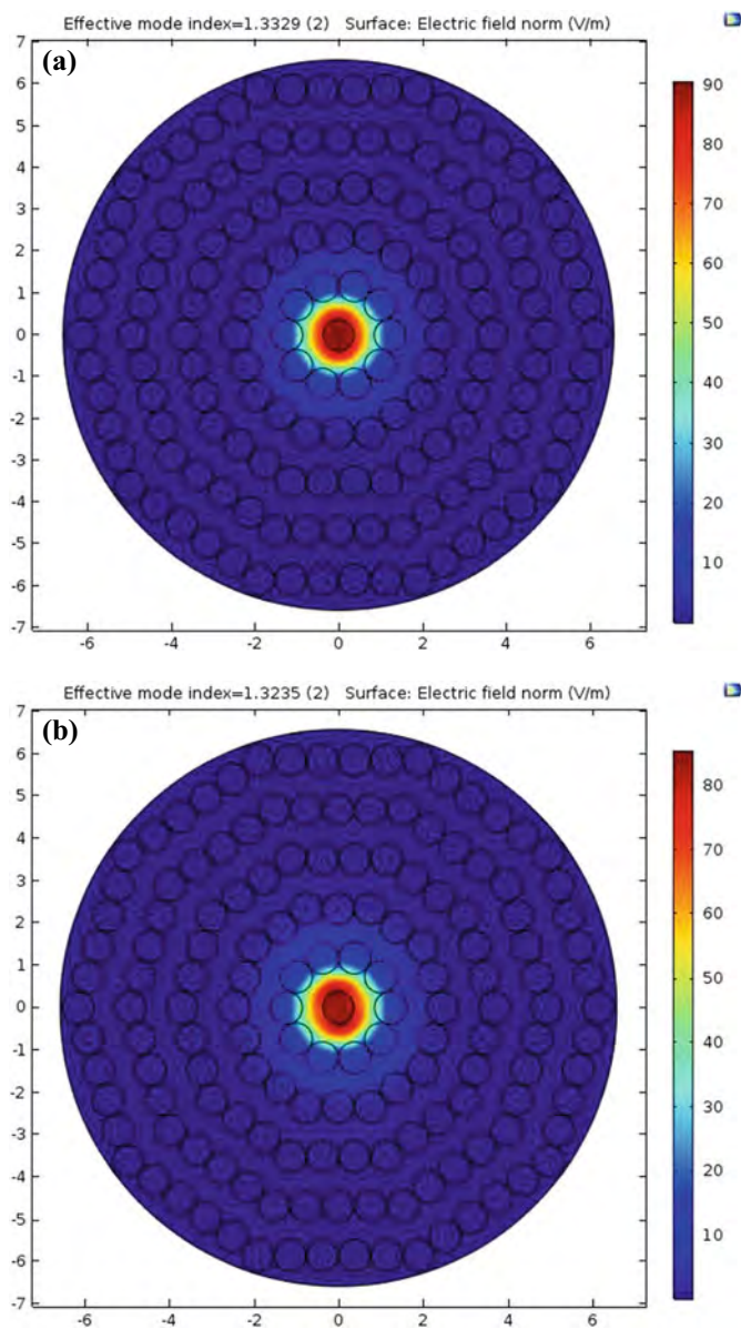
Fig. 2 a Snapshot of the modal intensity distribution of fundamental mode at 1.33\ \mu\text{m} when the core is filled with ethanol (1.354). b Snapshot of modal intensity distribution of fundamental mode at 1.33\ \mu\text{m} when core is filled with water (1.33)
