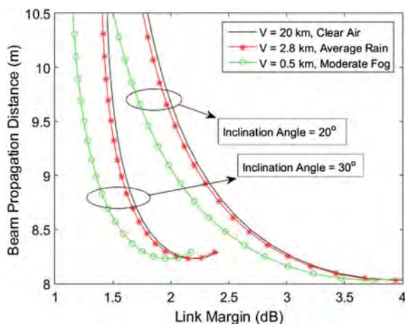
Fig. 6 Beam propagation distance against the available FSO link margin in different weather
