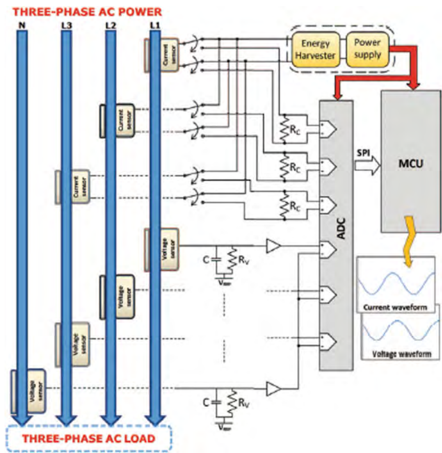
Fig. 5 Basic schematics of the meter with energy harvesting. As illustrated in [4, Fig. 2]
