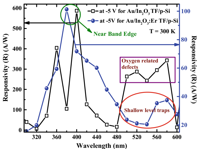
Fig. 3 Responsivity at different wavelengths for both the devices
