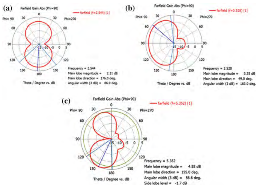
Fig. 4 Polar Radiation patterns of antenna at a 2.52 GHz b 3.5 GHz c 5.4 GHz
