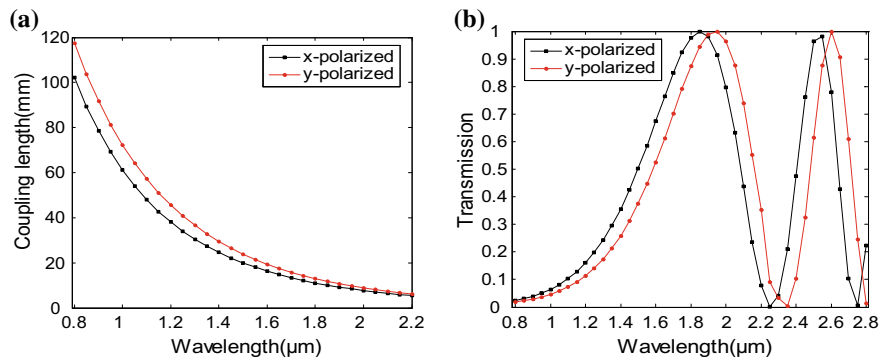
Fig. 4 a Coupling length variation of the x - and y -polarized light with wavelength when analyte refractive index n_a = 1.33 and hole diameter d = 3.0\text{ }\mu\text{m} , b transmission curve of dual-core PCF with a length of 1 cm
