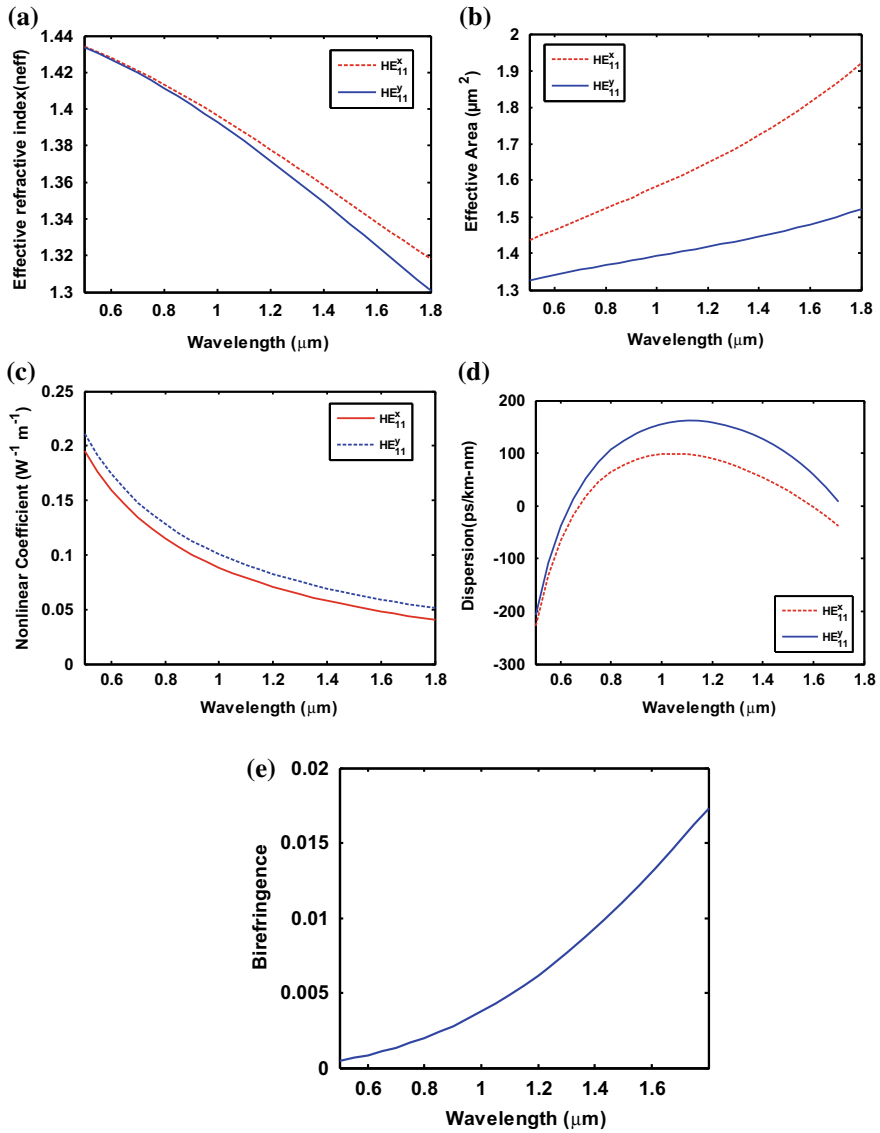
Fig. 2 a The effective index of proposed PCF ( n_{eff} ), b the effective area of PCF ( A_{eff} ), c nonlinear coefficient ( \gamma ), d dispersion curves for orthogonal modes and e birefringence (B)
