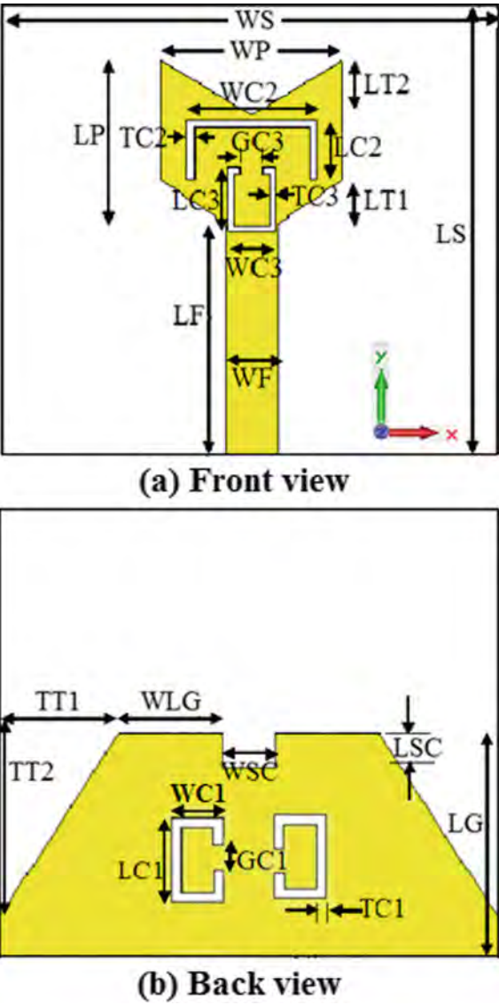
Fig. 2 Geometry of the proposed Y-shaped antenna a front view b back view
