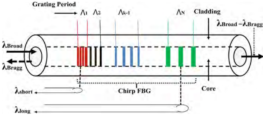
Fig. 1 Configuration of a chirped fiber Bragg grating used as a dispersion compensator
