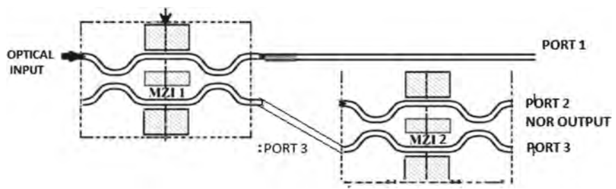
Fig. 5 Implementation blocks of NOR. Reproduced from [7]
