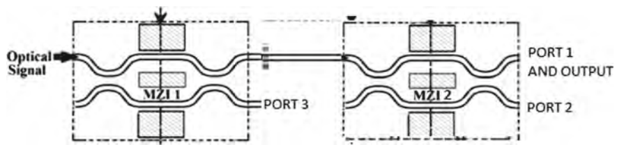
Fig. 3 Implementation blocks of AND gate. Reproduced from [3]
