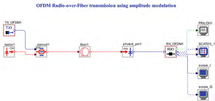
Fig. 2 OFDM over optical fiber transmission
