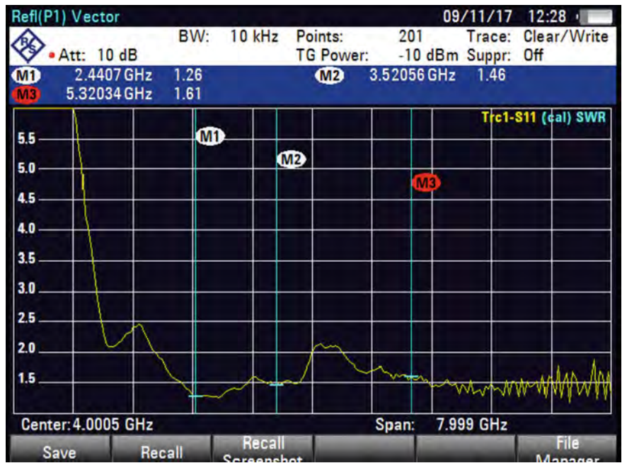
Fig. 8 Measured of VSWR
