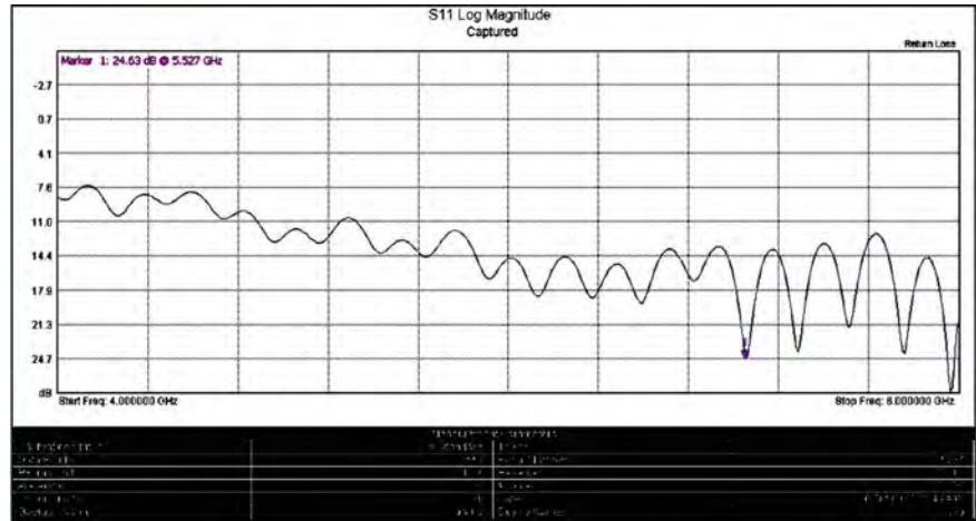
Fig. 15 VNA result of return loss with DGS
