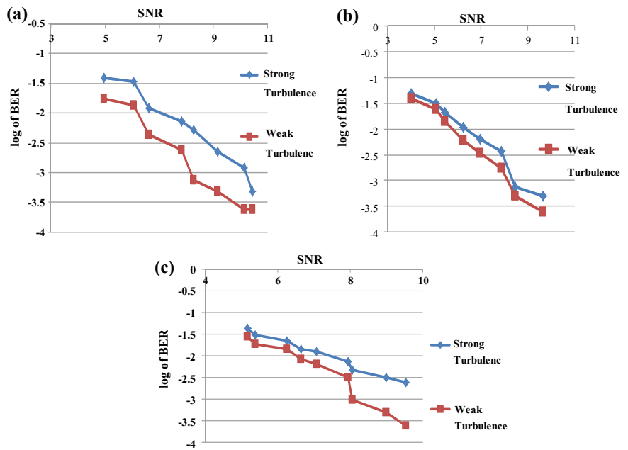
Fig. 4 Log of BER with SNR relation a BER performance in heavy rainy days, b BER performance in light rainy days and c BER performance in hazy days
