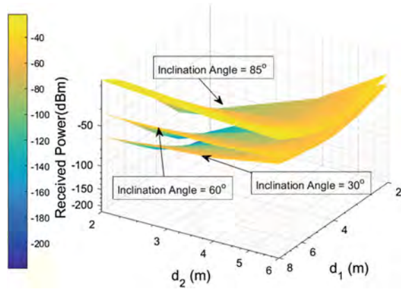
Fig. 4 3-D schematic illustrating the received power profile for varying horizontal and vertical separation distance, L = 1 m
