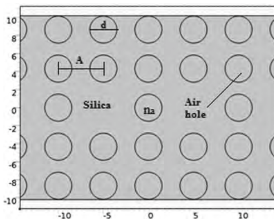
Fig. 1 Geometry of the proposed dual-core photonic crystal fiber
