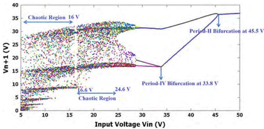
Fig.2 Bifurcation diagram
