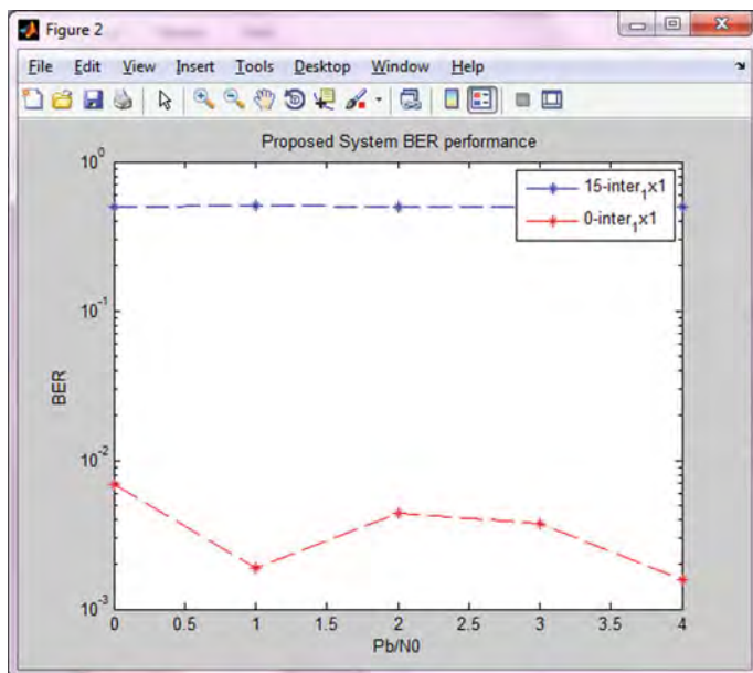
Fig. 10 SNR versus BER with various noise interference
