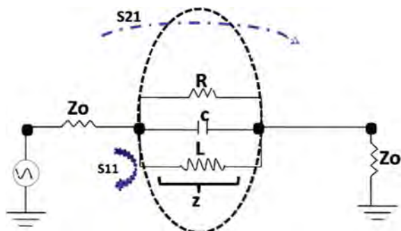
Fig. 1 Equivalent circuit of DGS
