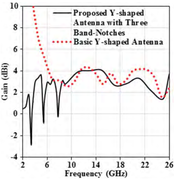
Fig. 8 Gain comparison for proposed Y-shaped antenna with three band notches and basic Y-shaped antenna
