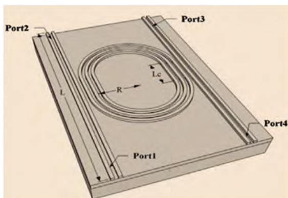
Fig. 6 Three dimensional structure view of double slot waveguide ring resonator. Reproduced from Ref. [28]
