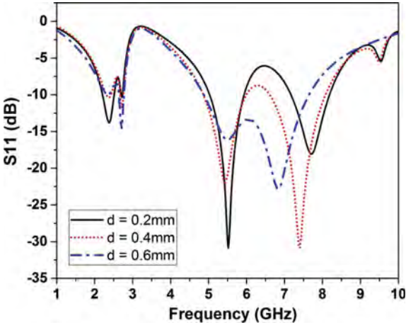
Fig. 5 Comparison of reflection coefficients for varying distance “d” between feed and the ground at d = 0.2 mm, d = 0.4 mm, and d = 0.6 mm
