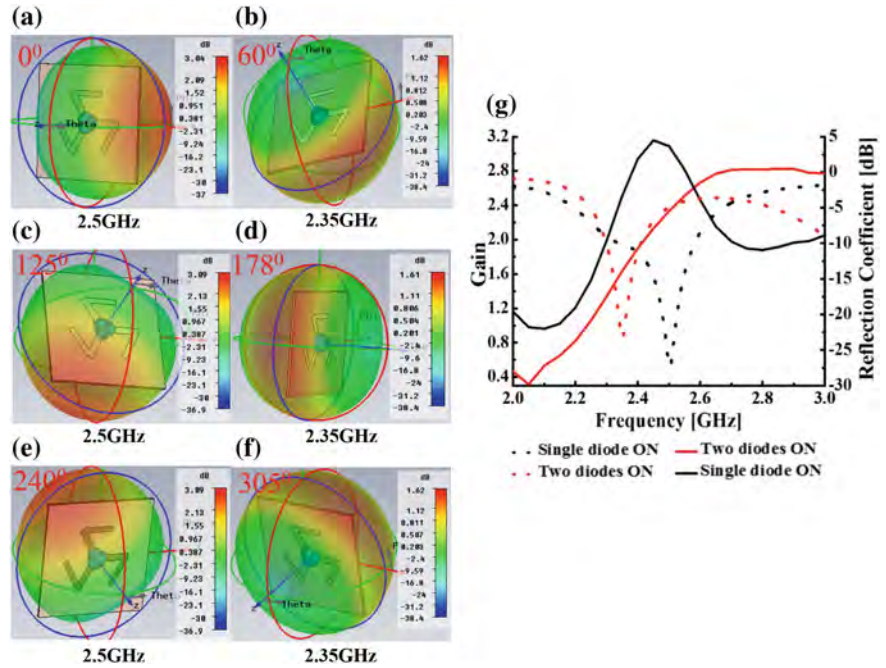
Fig. 3 Radiation pattern of antenna in azimuth plane XY ( \theta = 90^\circ ) when diode a D_1 is ON, b D_1 and D_2 are ON, c D_2 is ON, d D_2 and D_3 are ON, e D_3 is ON, f D_3 and D_1 are ON, g plot showing gain pattern and reflection coefficient of antenna
