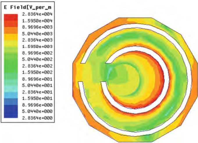
Fig. 5 Current distribution at frequency of 14 GHz
