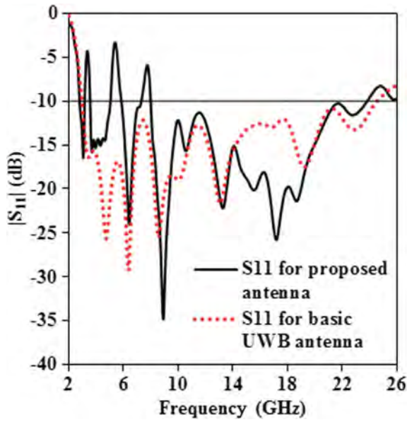
Fig. 4 Comparison of magnitude of S_{11} plot for basic Y-shaped antenna and the proposed Y-shaped antenna with three band notches
