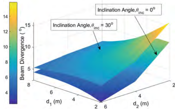
Fig. 3 3-D schematic illustrating optimum source beam divergence angle for varying horizontal and vertical separation distances, L = 1 m
