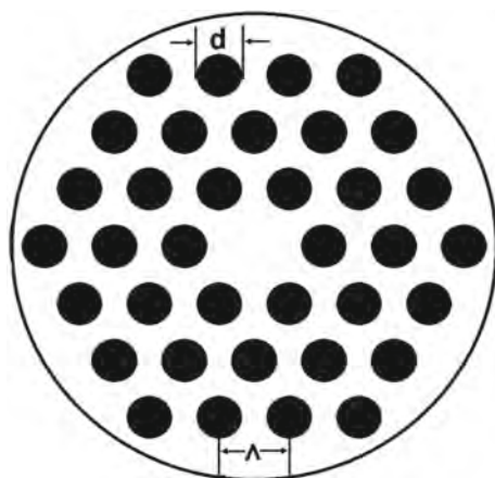
Fig. 1 Schematic view of the designed PCF
